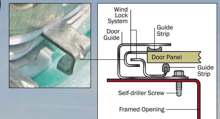
SERIES TMB 5000 Door Engagement Detail
