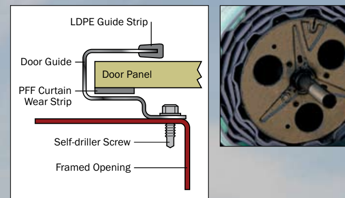
SERIES TMB 2500 Door Engagement Detail
