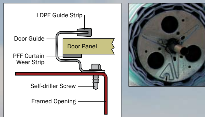
SERIES TMB 2000 Door Engagement Detail
